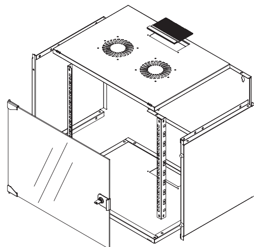
Exploded view
