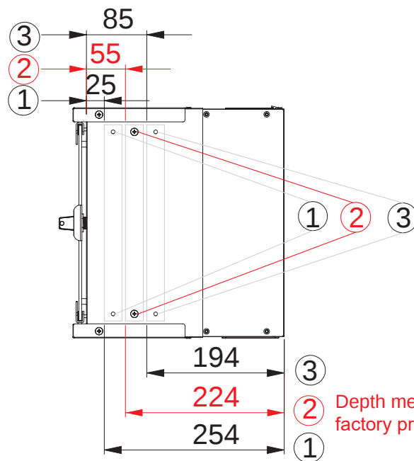
19" mounting top view
