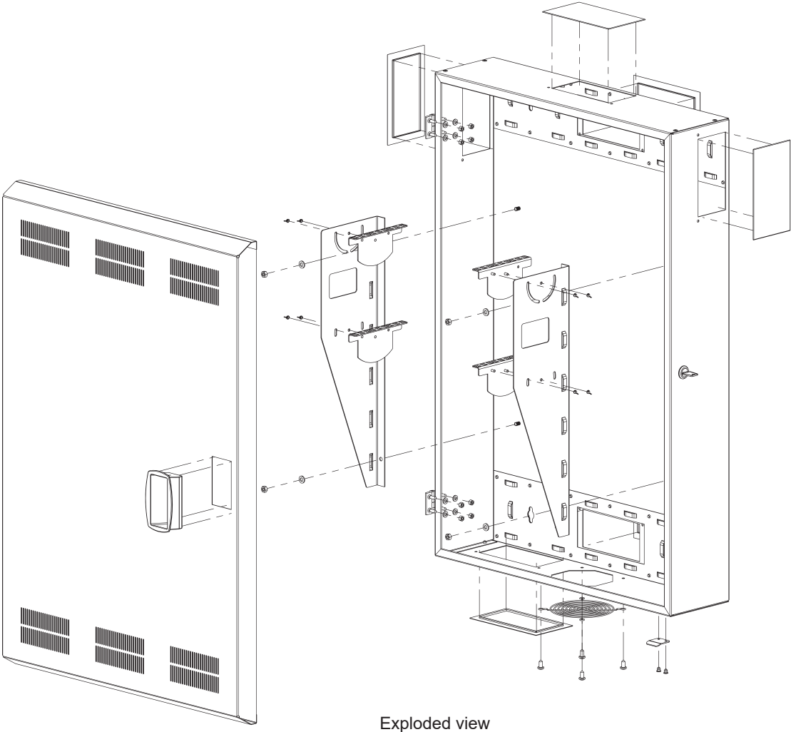
Exploded view
