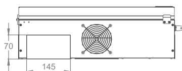
Bottom view
