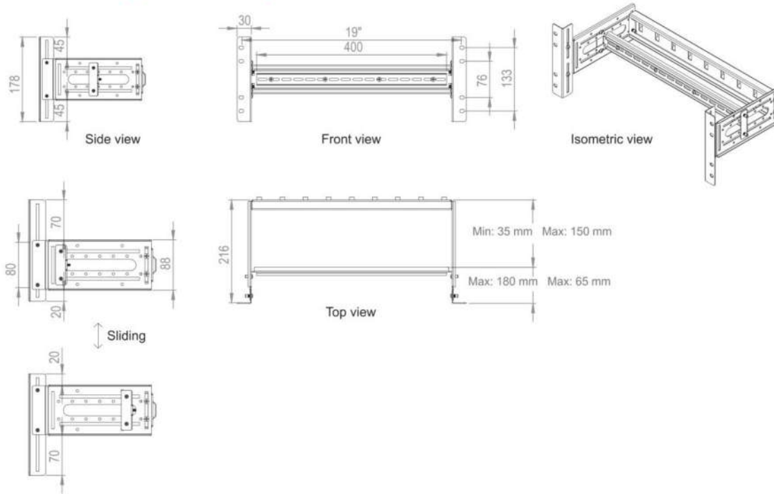
DIN Rail depth adjustment stepless
