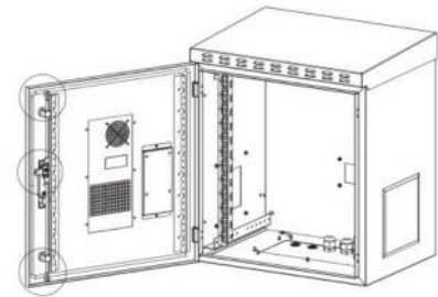
3 point locking system
