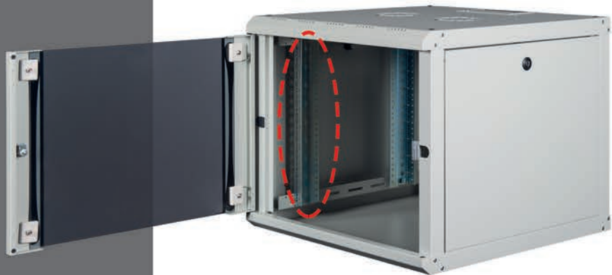
Threaded 19" Rack Rails for M5 Screw
