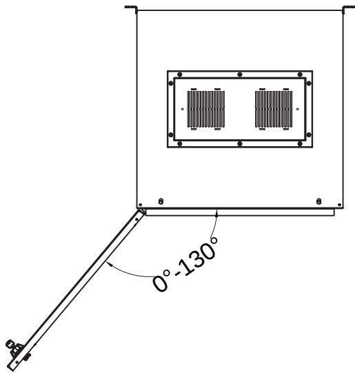
Front door opening angle
