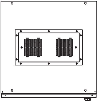
Interior view-Top
