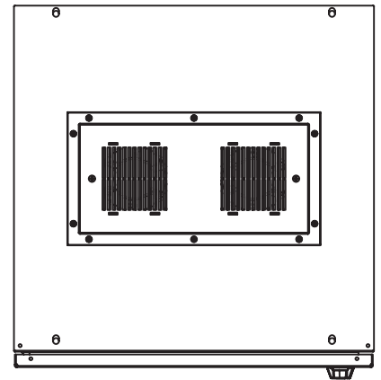
Interior view-Top
