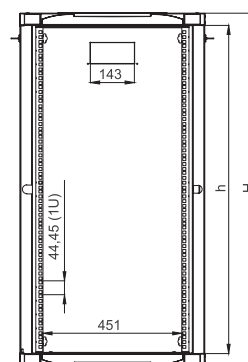
Dimensions in width and height
