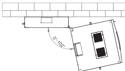
Double section wall opening angle
