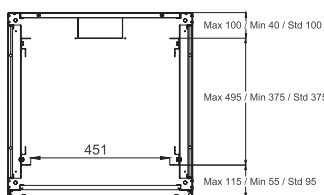
Max / Min / Std Equipment mounting distance
