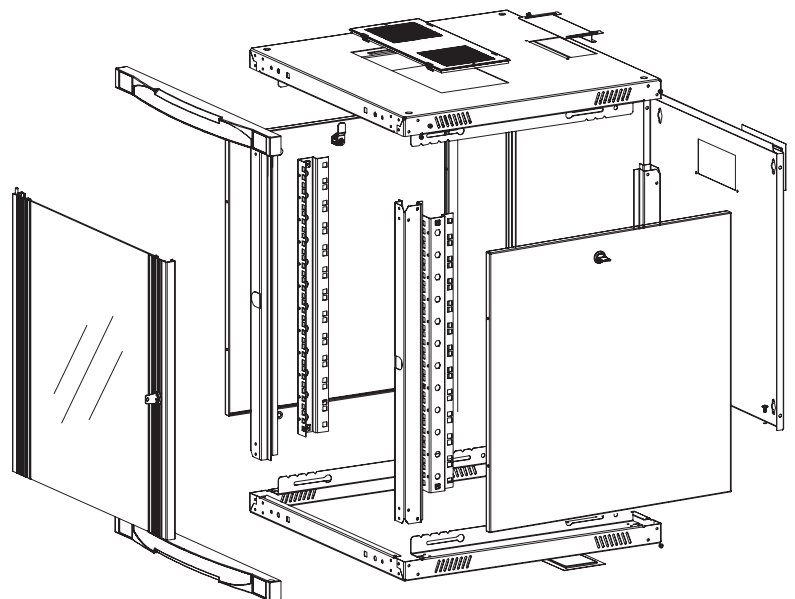
Exploded view
