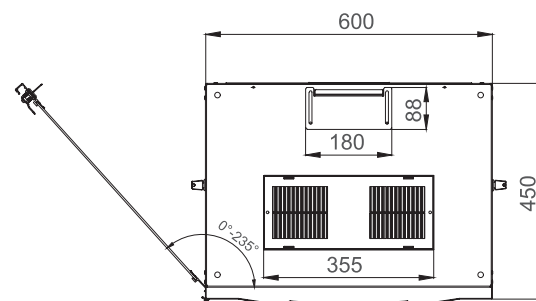
Dimensions in width and height
