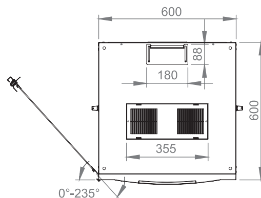
Dimensions in width and height
