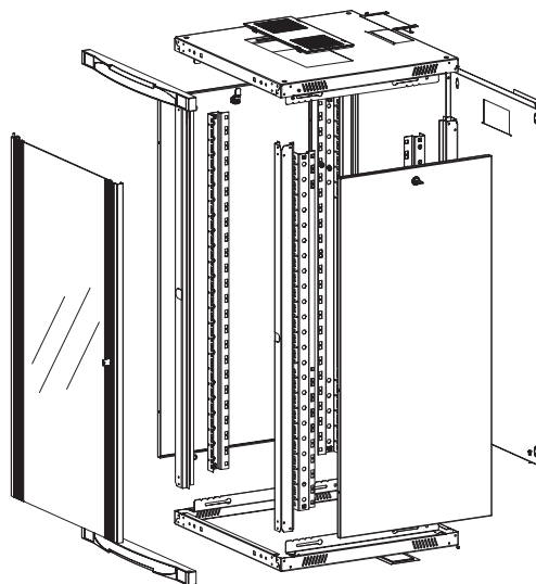
Exploded view
