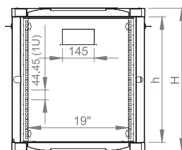
Max. / Std. / Min. Equipment mounting distance
