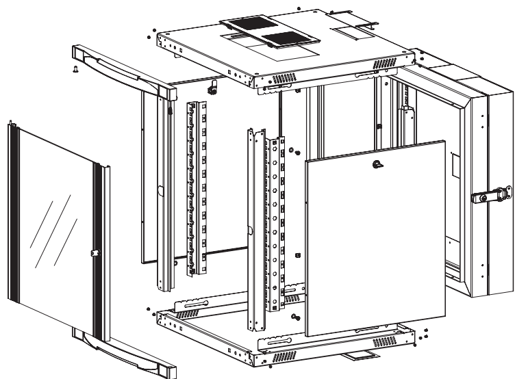
Exploded view
