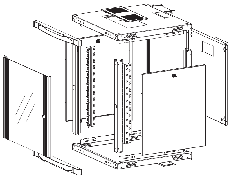
Exploded view
