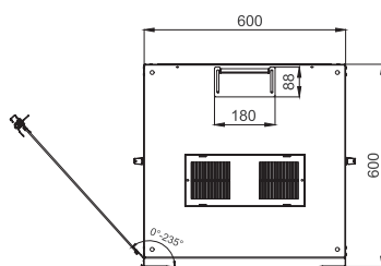
Front door opening angle
