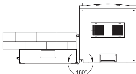
Double section column opening angle
