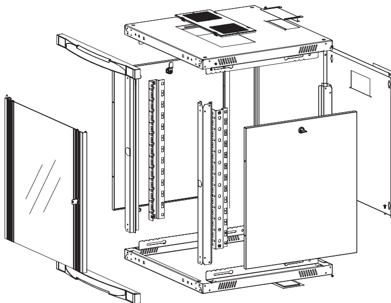
Exploded view
