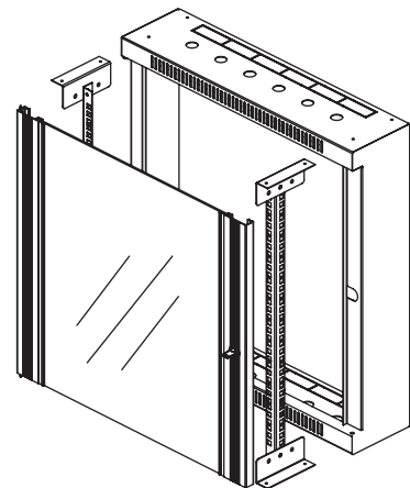
Exploded view
