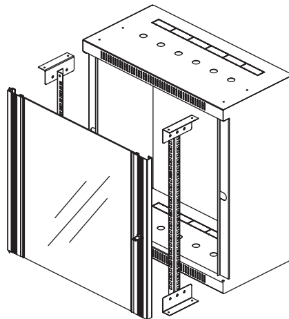
Exploded view
