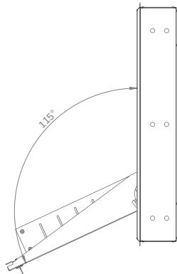
Open in service position: 115° Second stopper position
