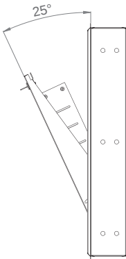
Open in operation position: 25° First stopper position
