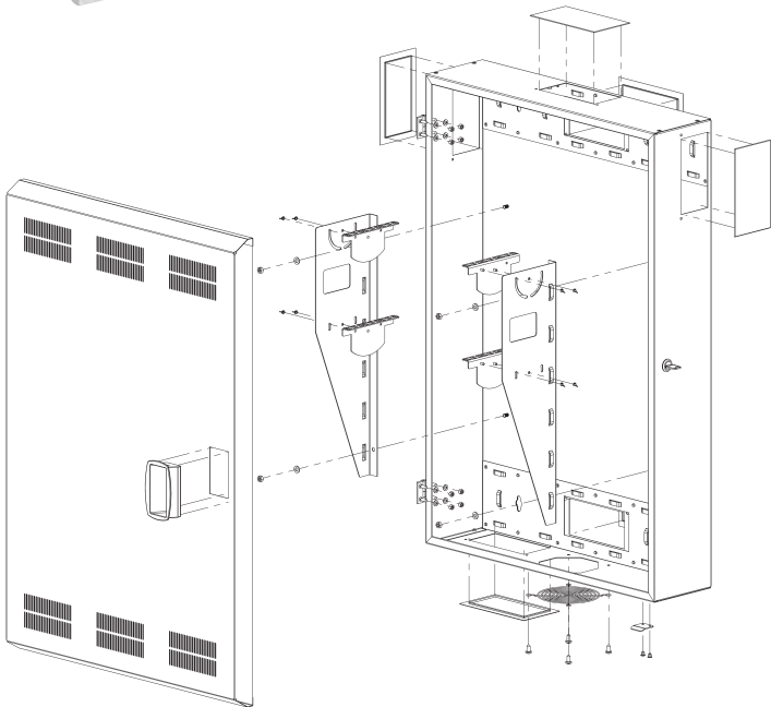
Exploded view
