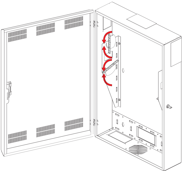
Both rack rails can be adjusted 100°
