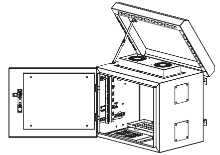
FRONT DOOR AND TOP COVER OPEN, ISOMETRIC VIEW
