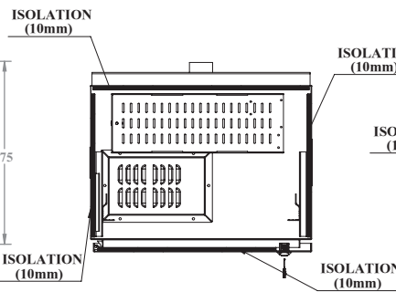
UPPER DETAILED VIEW
