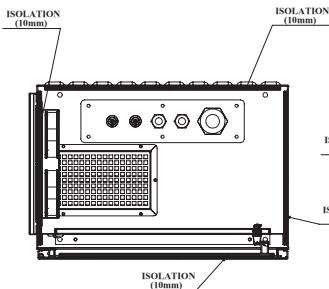
UPPER DETAILED VIEW
