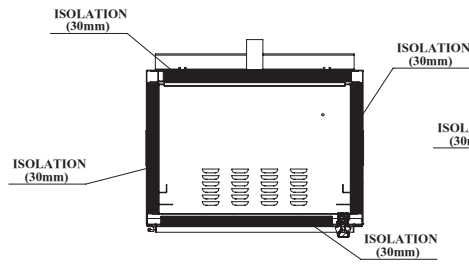
UPPER VIEW
