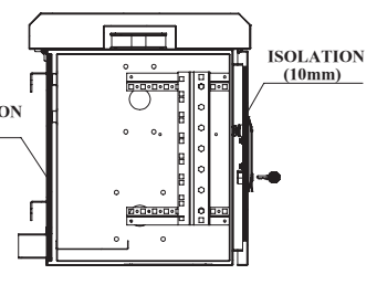
SIDE DETAILED VIEW
