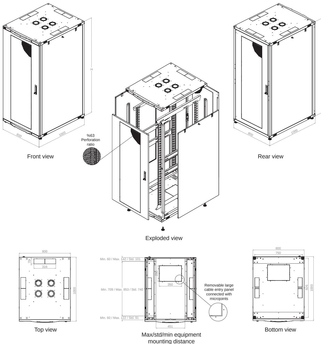
19" CK-Line Free Standing CS Model Server Cabinets W=800 mm D=1000 mm
