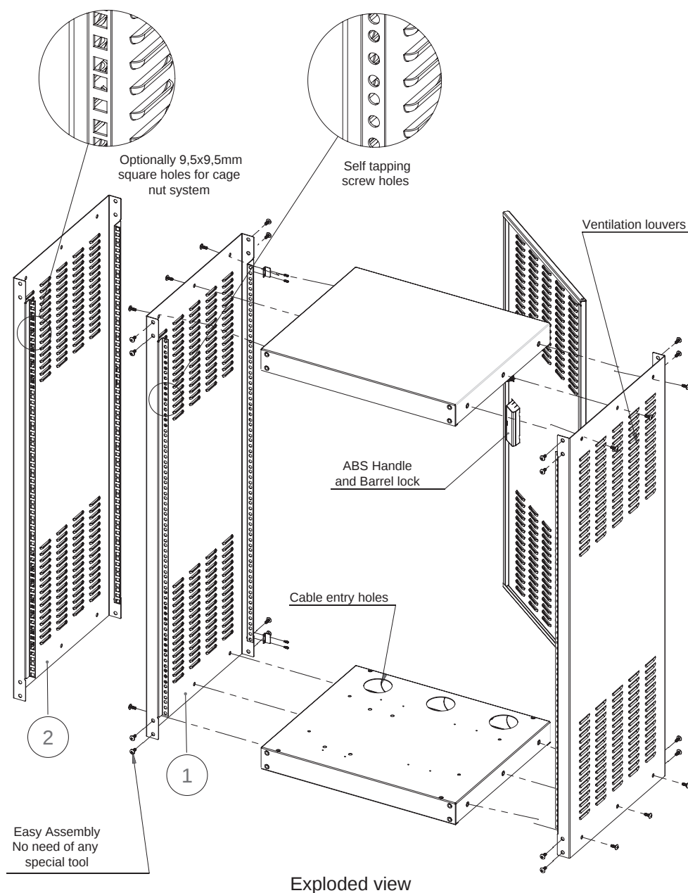
19" Audio Video AVS Cabinets W:557 mm D:470 mm
