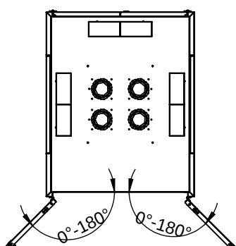
Front door Opening view
