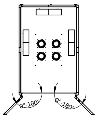
Front door Opening view
