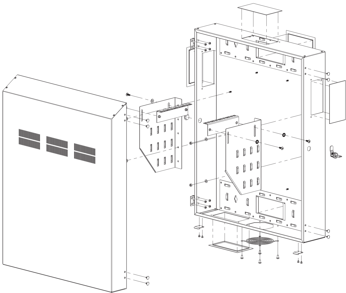
Exploded view
