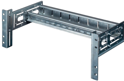
4U Mounting 19" ears, DIN rail set to middle position, 19" rails adjusted to top elevation.
