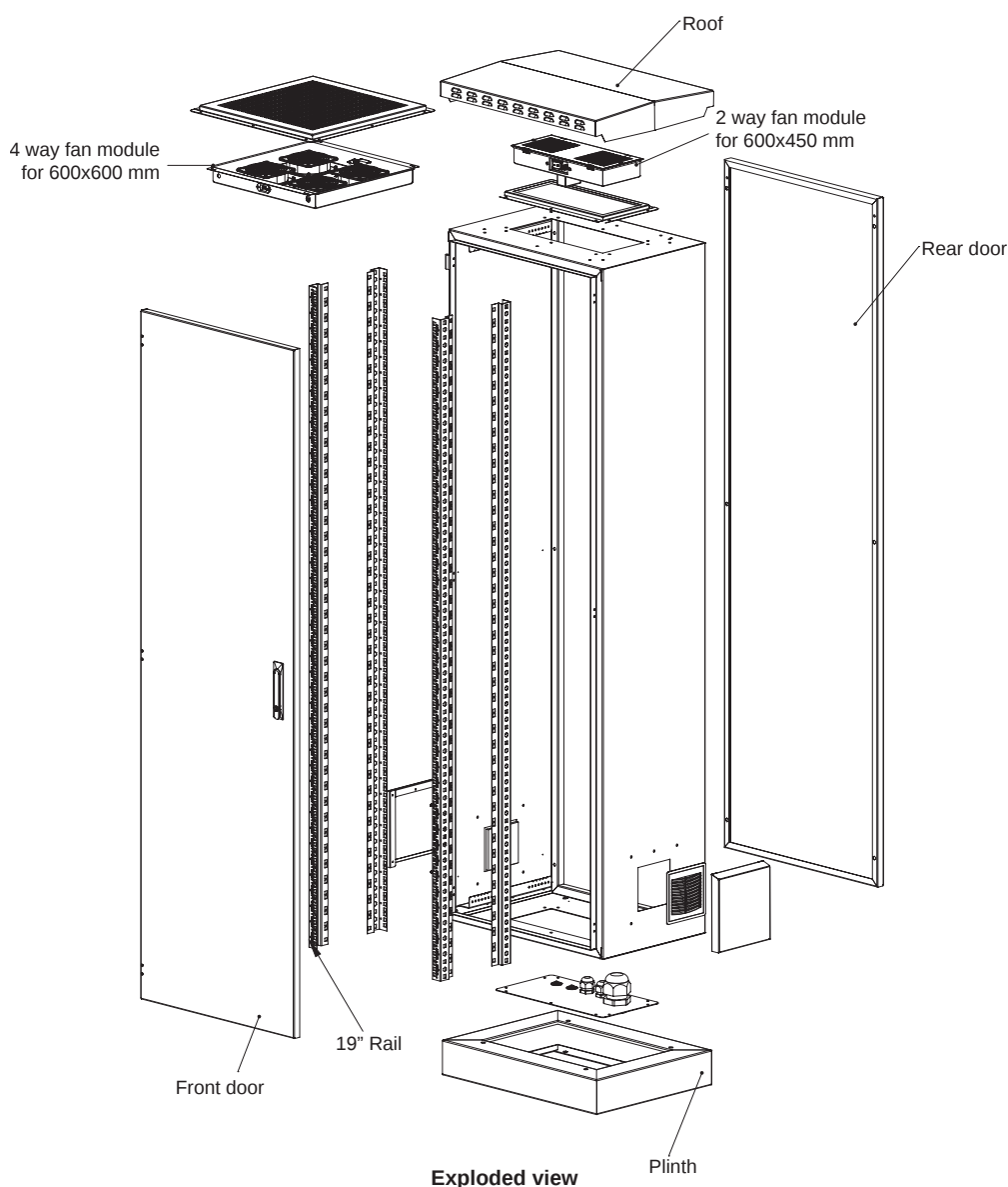
Exploded view
