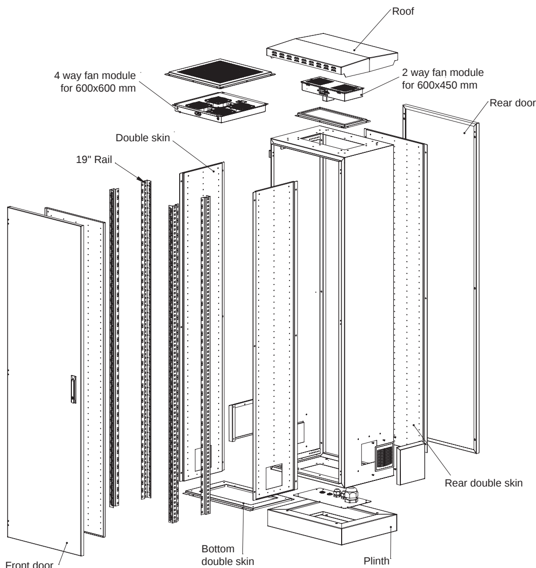
Exploded view
