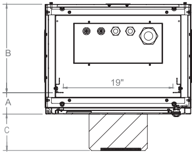
Top inside view
