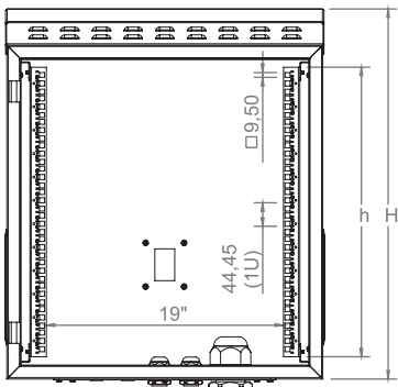
Inside view
