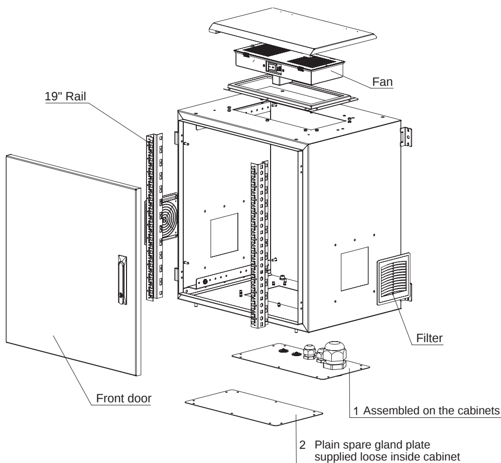
Exploded view
