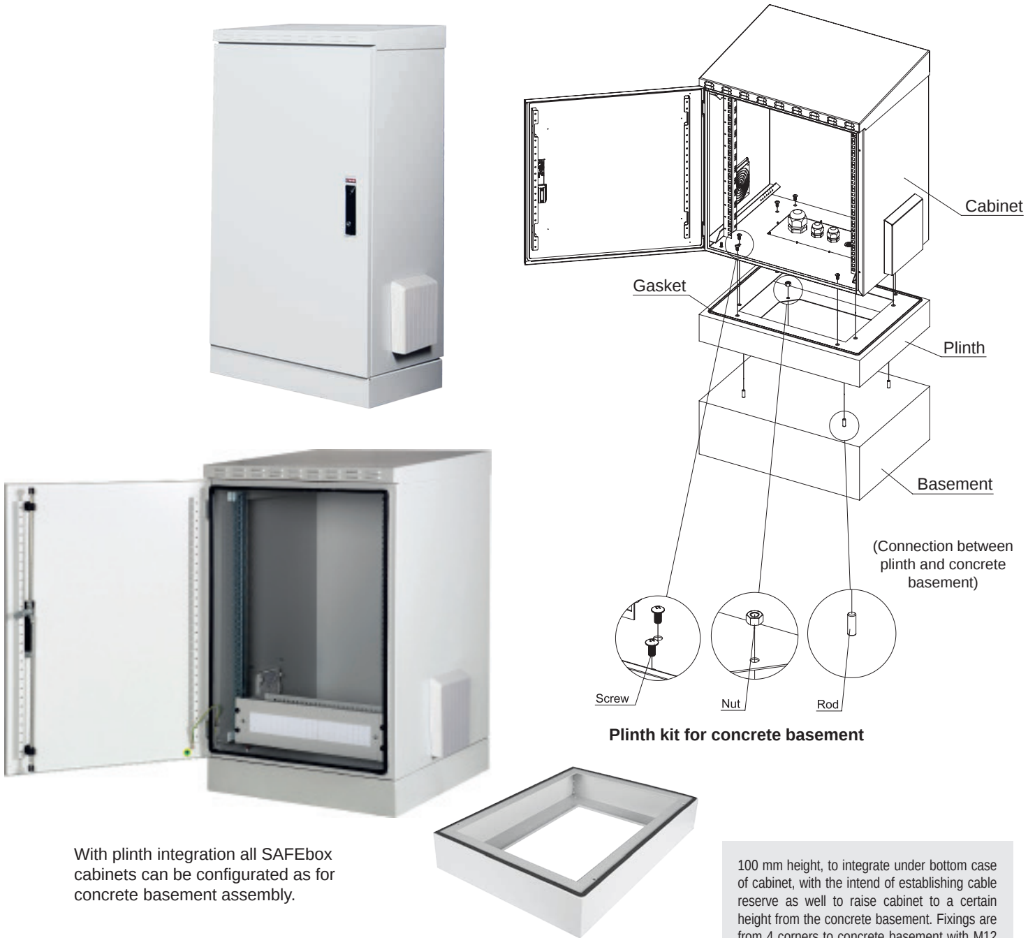
SAFEbox Series IP55 Outdoor Plinth for Concrete Assembly
