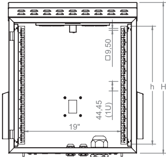
Inside view
