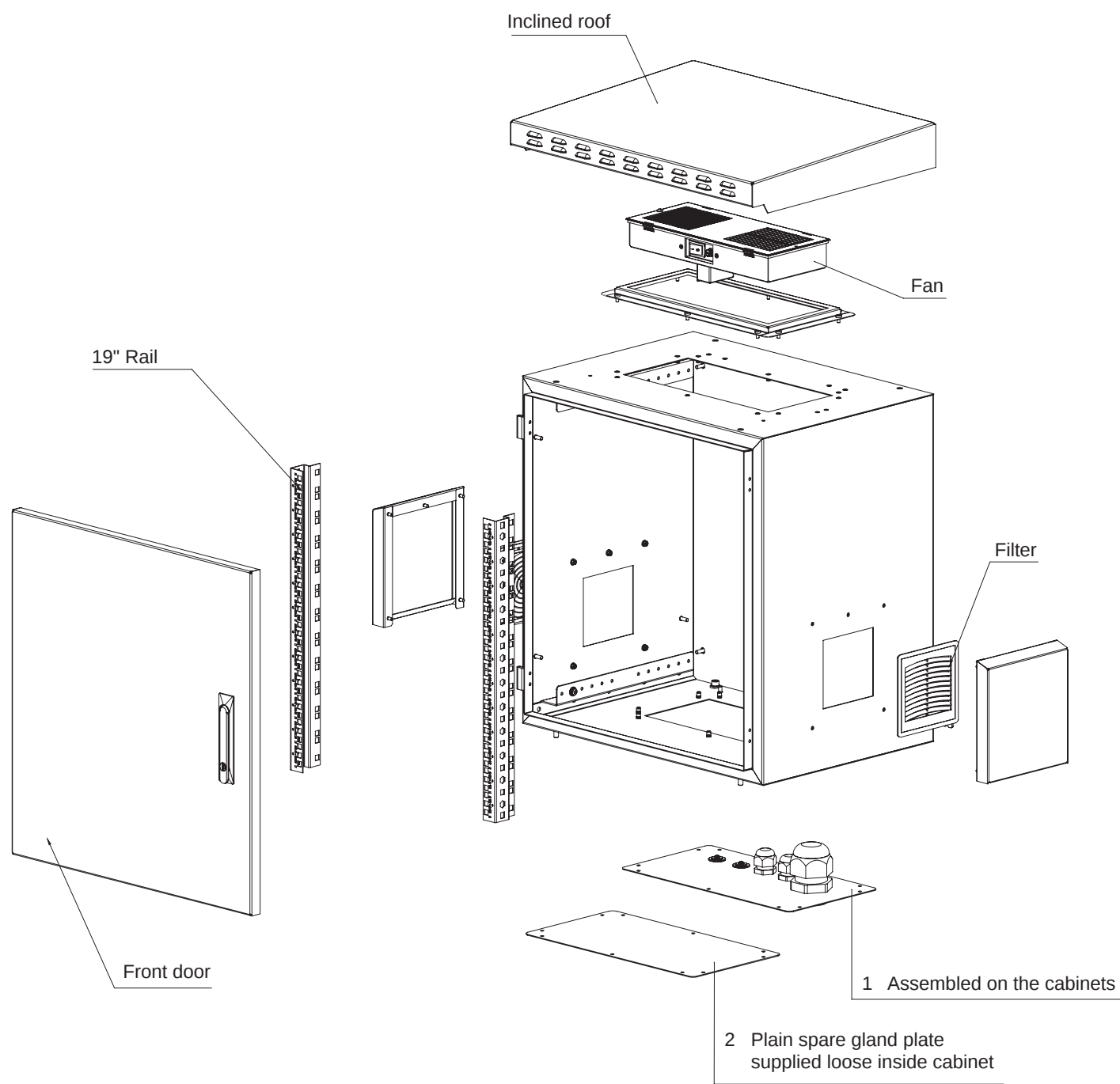
Exploded view
