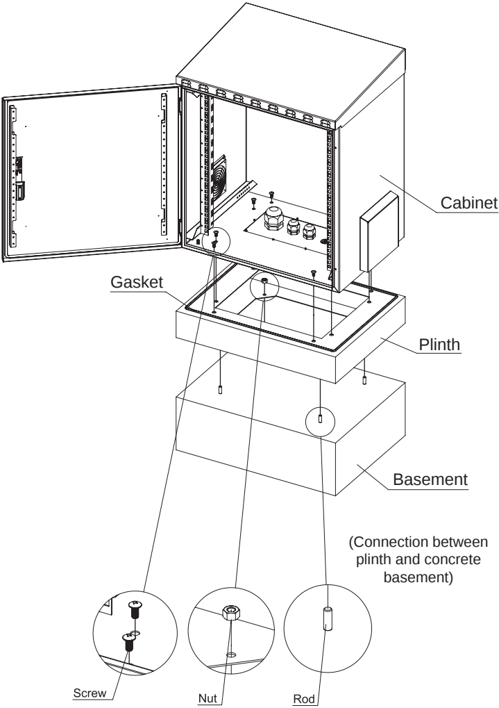
Plinth kit for concrete basement
