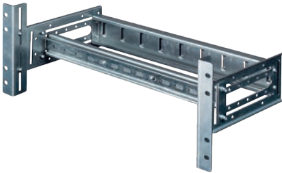
4U Mounting 19" ears, DIN rail set to front, 19" rails adjusted to middle elevation.
