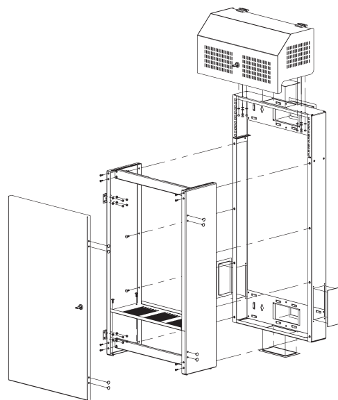
Exploded view
