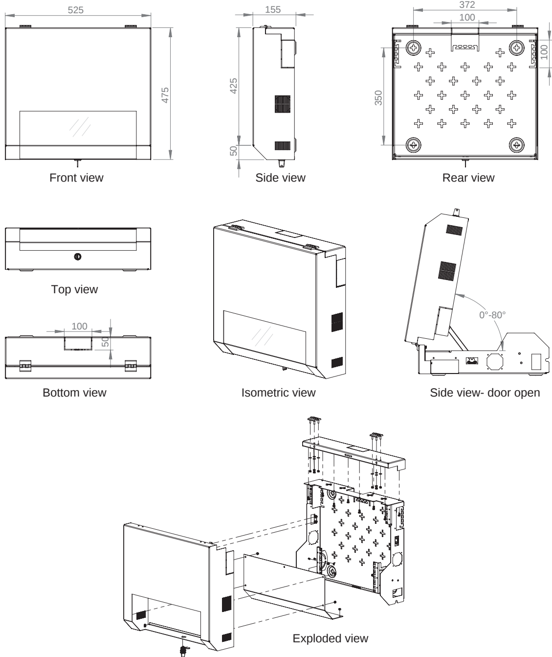
19" SLIMbox MODEL 1 Hinged Cover Series Wall Mounting Cabinets W:500 mm D:475 mm H:155 mm
