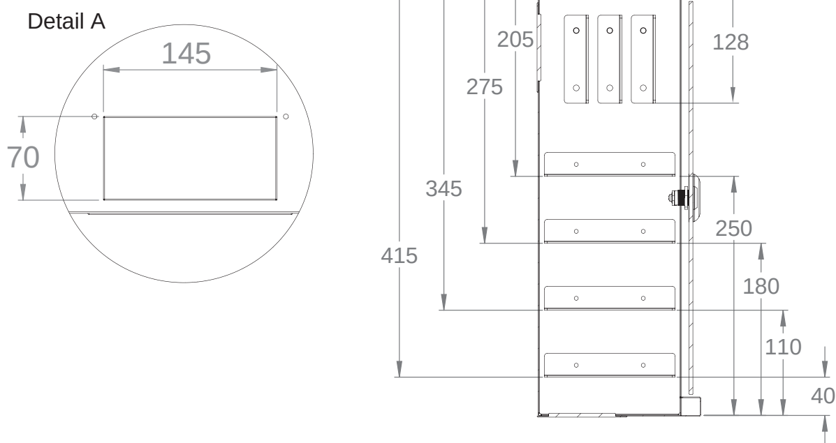
3U 19" mounting rails side view
