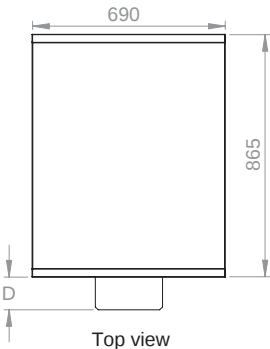
IP65 Outdoor 600x800 mm Air Conditioned
